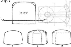
Three types of crown covering. (1) Material in one-piece steamed to the shape of crown. (2) Sections sewn together. (3) Side crown and tip covered separately
